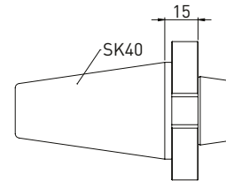
Order No. Name 350130014 Adapter SK40 on Haas/Walter taper
